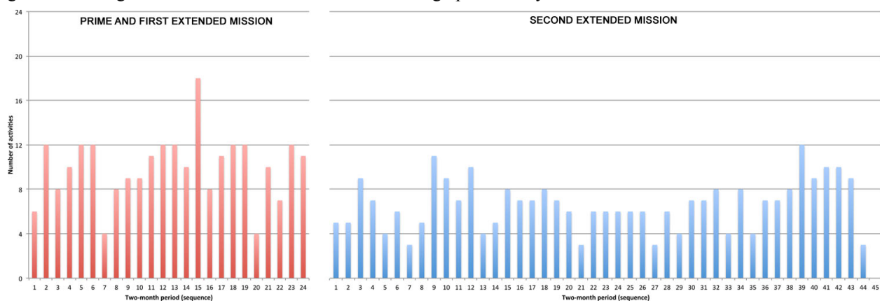
Figure 4. Cassini activity intensity, expressed as a number of intensive events per sequence
