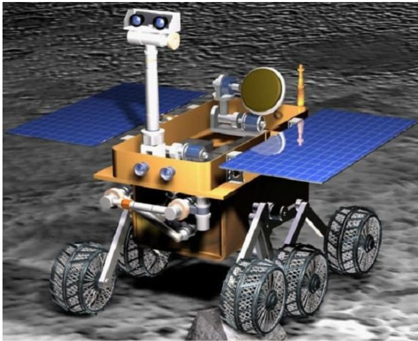
Figure 1 the rover model
