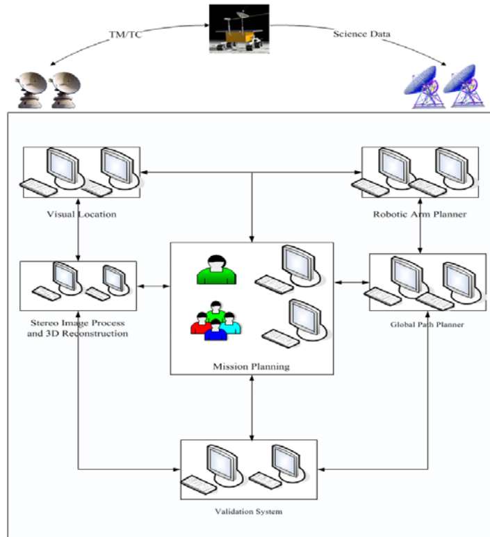
Fig 4 the overall architecture of the teleoperation system
