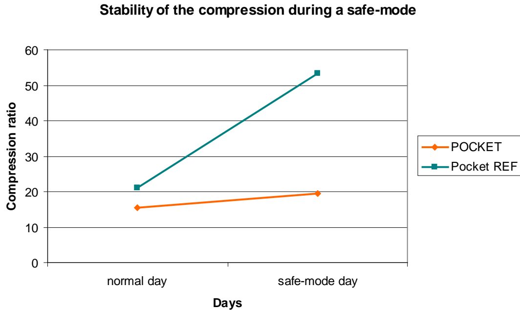
Figure 5. Compression performance comparison of POCKET and POCKET REFERENCE after a safe-mode entry. The figure shows that the compression ratio of POCKET remains noticeably stable during the safe-mode period, even when the mask packets and inversion/correlation instructions have not been updated. POCKET REFERENCE shows a substantial performance degradation, being more sensitive to status changes in the telemetry.
