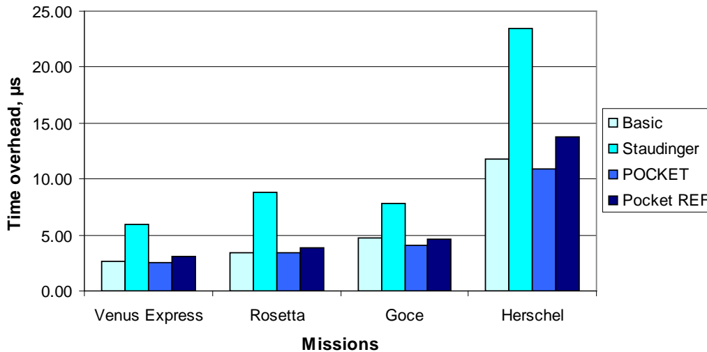
Figure 3. Speed performance comparison by mission for the four methods illustrated in sections V, VI, VII and VIII. The figure shows the average time, expressed in microseconds, needed to compress a packet of each mission on an Intel i7 notebook.
