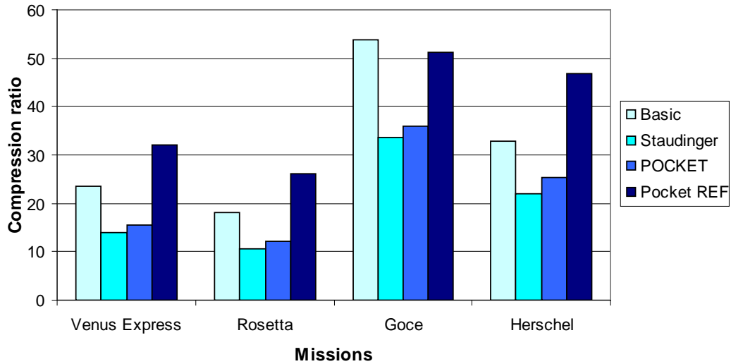
Figure 2. Compression performance comparison by mission for the four methods illustrated in sections V, VI, VII and VIII. The figure shows the compression ratio percentages by mission, as size of the compressed packets compared to the original packet stores. For every mission, a week's worth of stored housekeeping data has been considered.
